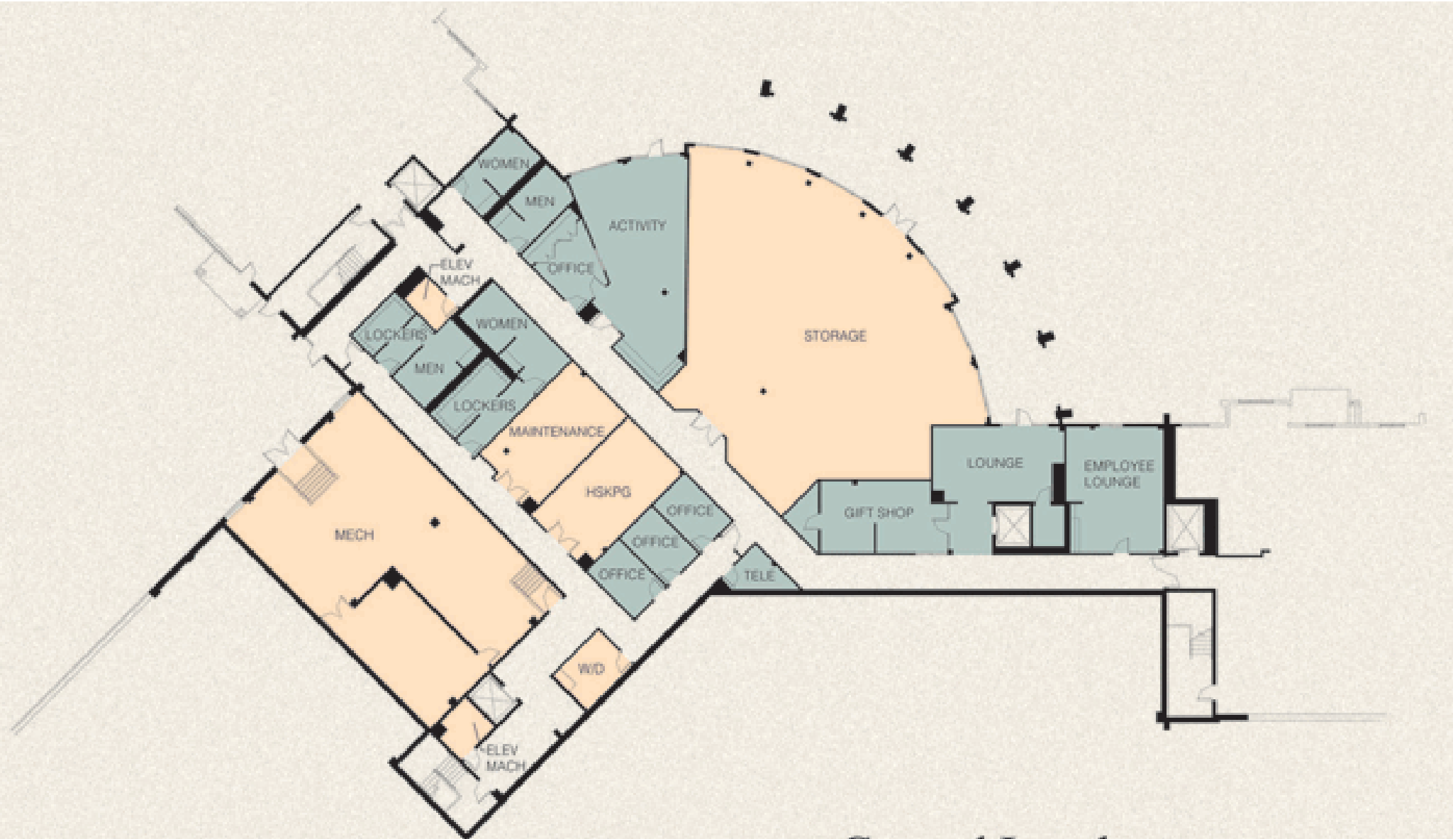
Ground Level
